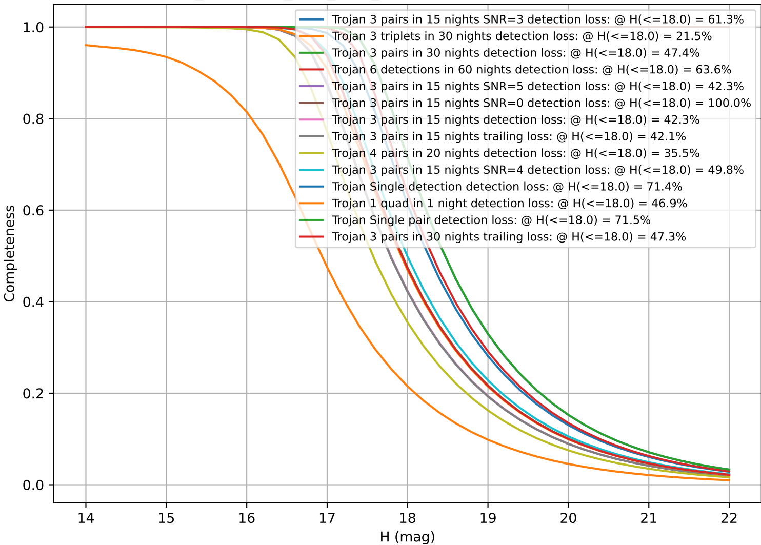
too_combined_s0.5_v3.4_10yrs: CumulativeCompleteness
