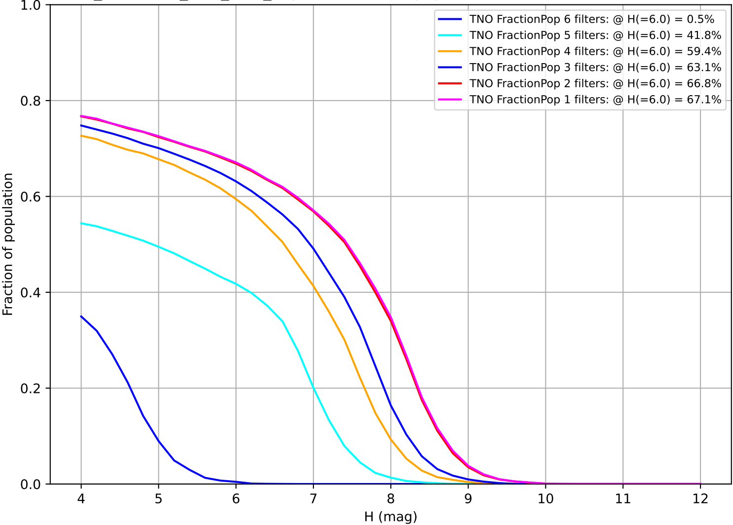
too_combined_s0.5_v3.4_10yrs: Fraction of population with colors in X filters TNO
