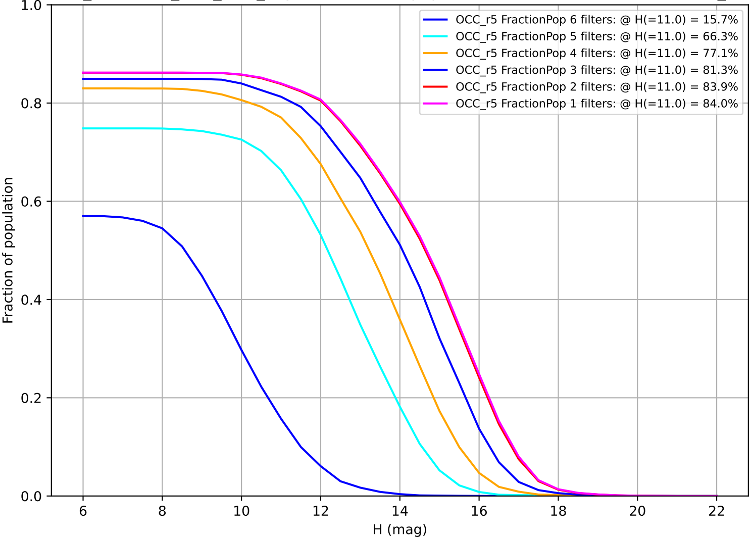
too_combined_s0.5_v3.4_10yrs: Fraction of population with colors in X filters OCC_r5
