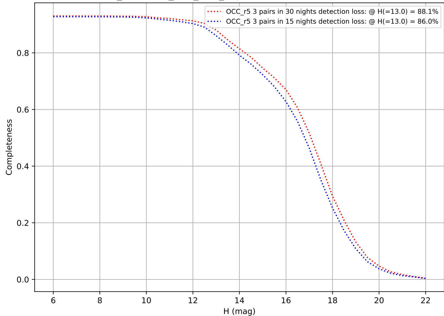
too_combined_s0.5_v3.4_10yrs: DifferentialCompleteness
