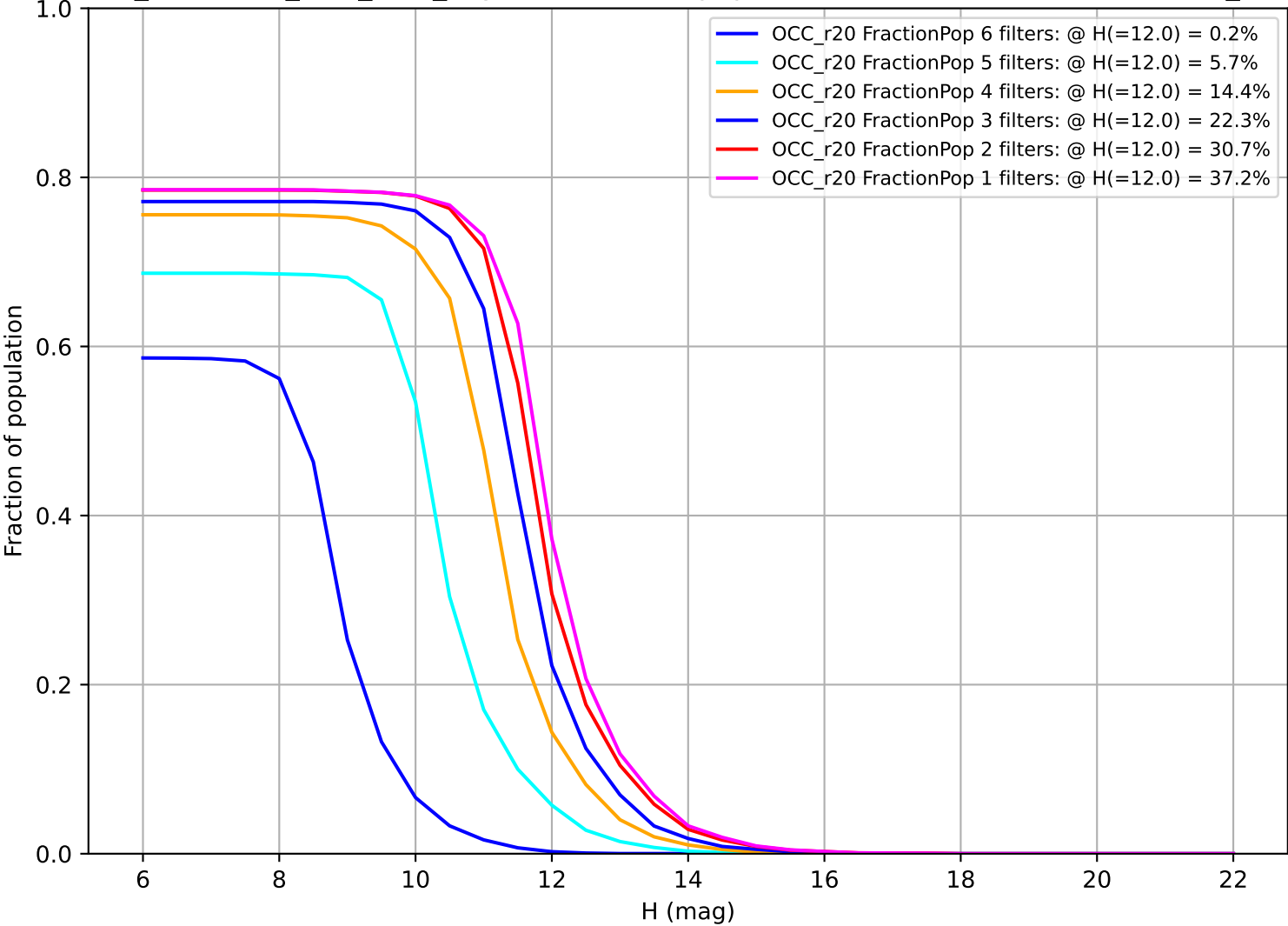
too_combined_s0.5_v3.4_10yrs: Fraction of population with colors in X filters OCC_r20
