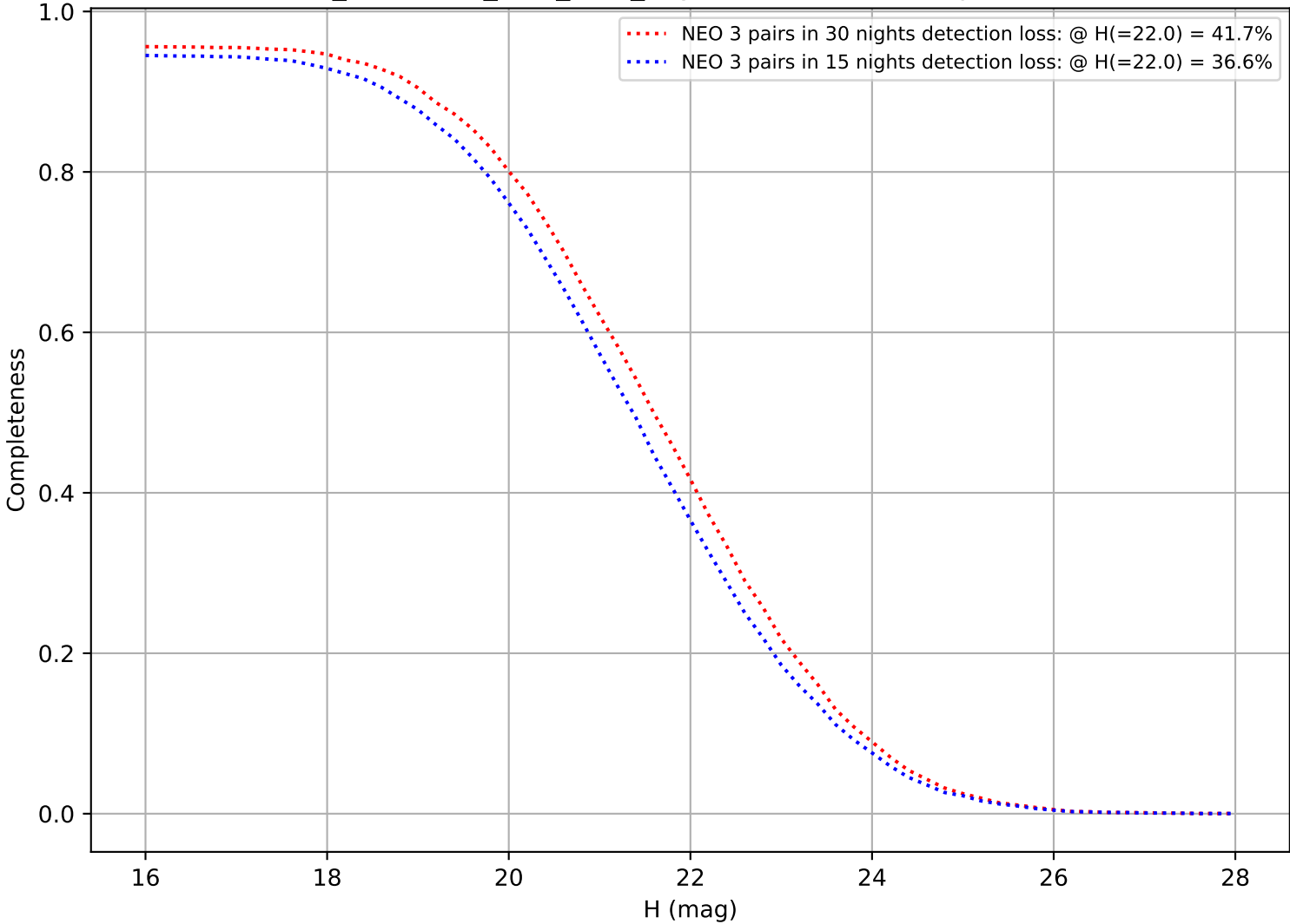
too_combined_s0.5_v3.4_10yrs: DifferentialCompleteness
