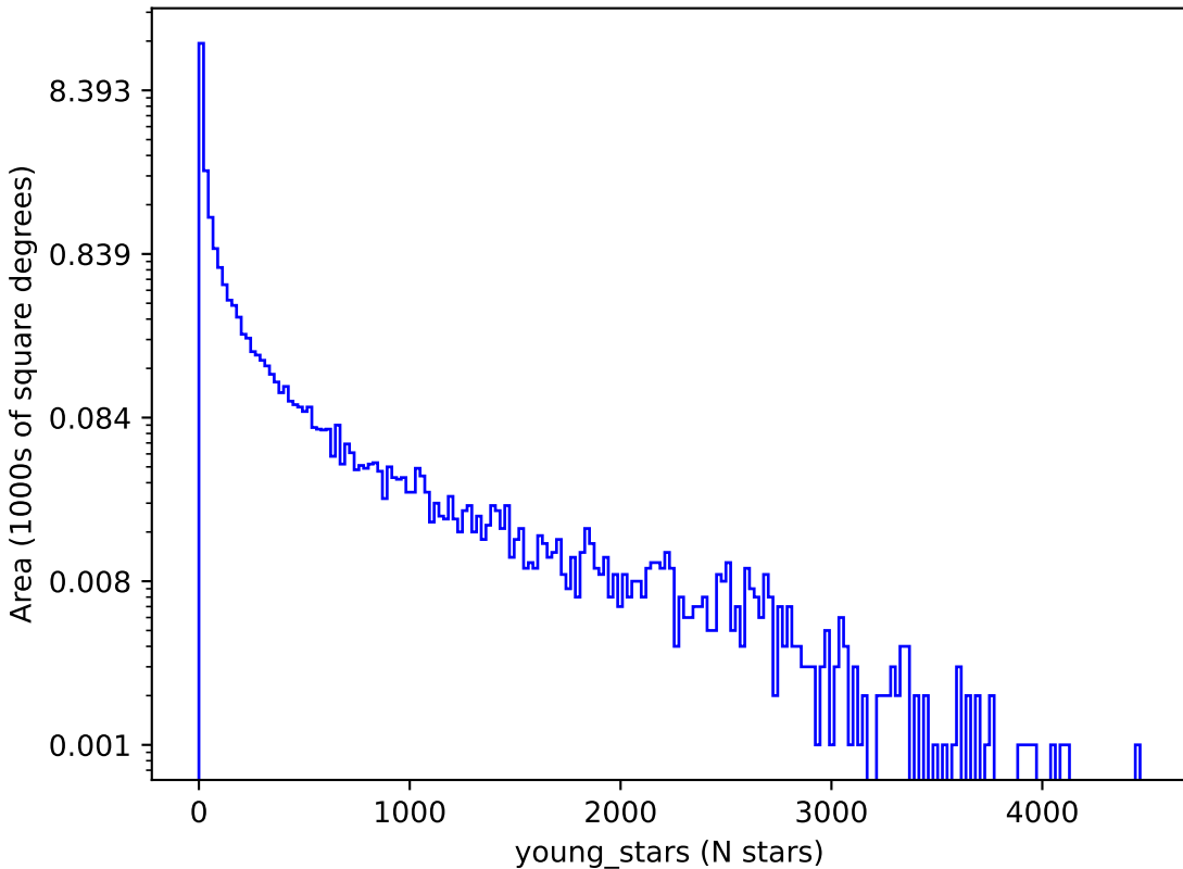
too_combined_s0.5_v3.4_10yrs : young_stars
