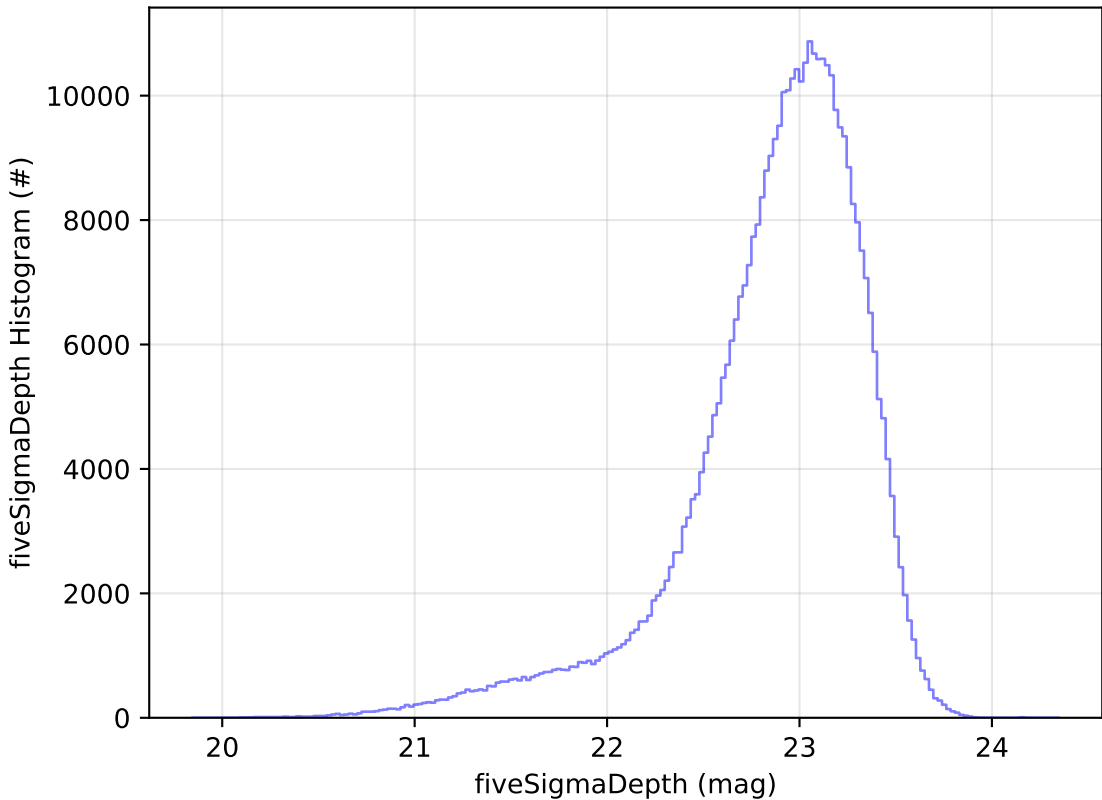
too_combined_s0.5_v3.4_10yrs z: fiveSigmaDepth Histogram
