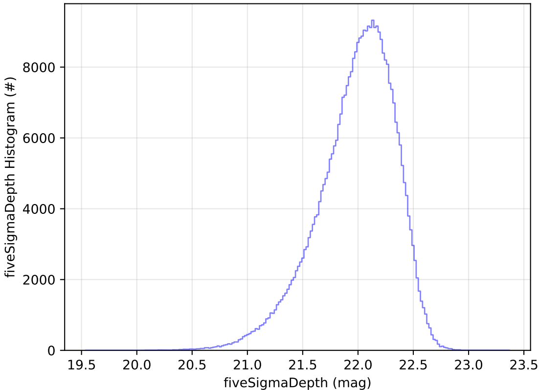
too_combined_s0.5_v3.4_10yrs y: fiveSigmaDepth Histogram
