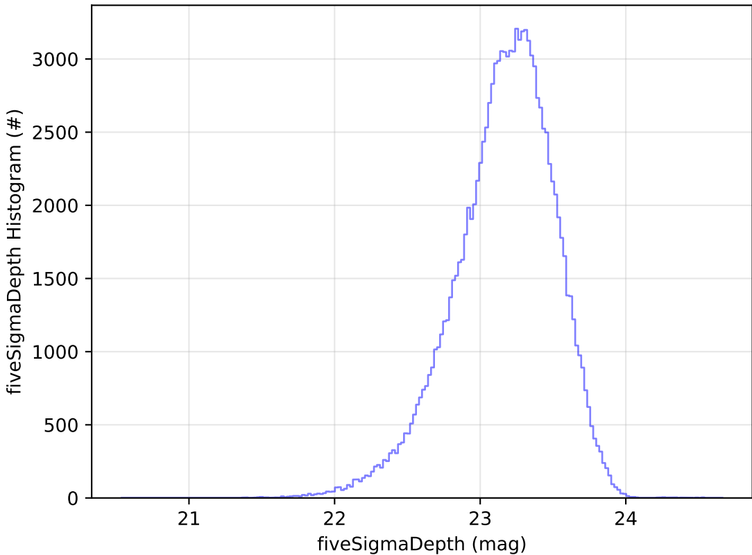
too_combined_s0.5_v3.4_10yrs u: fiveSigmaDepth Histogram
