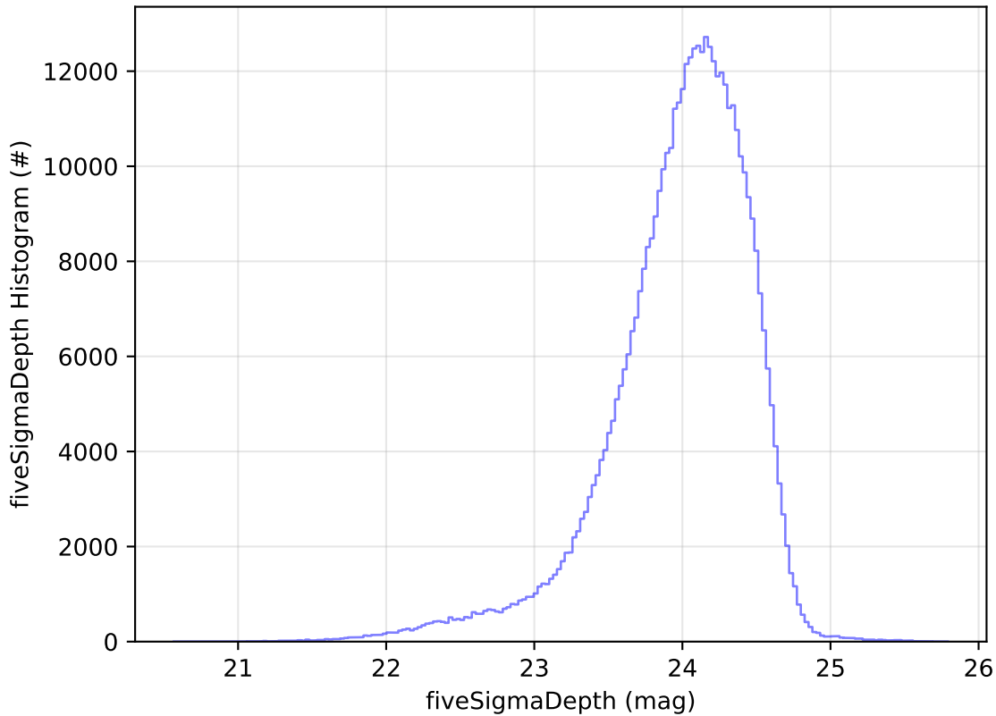
too_combined_s0.5_v3.4_10yrs r: fiveSigmaDepth Histogram
