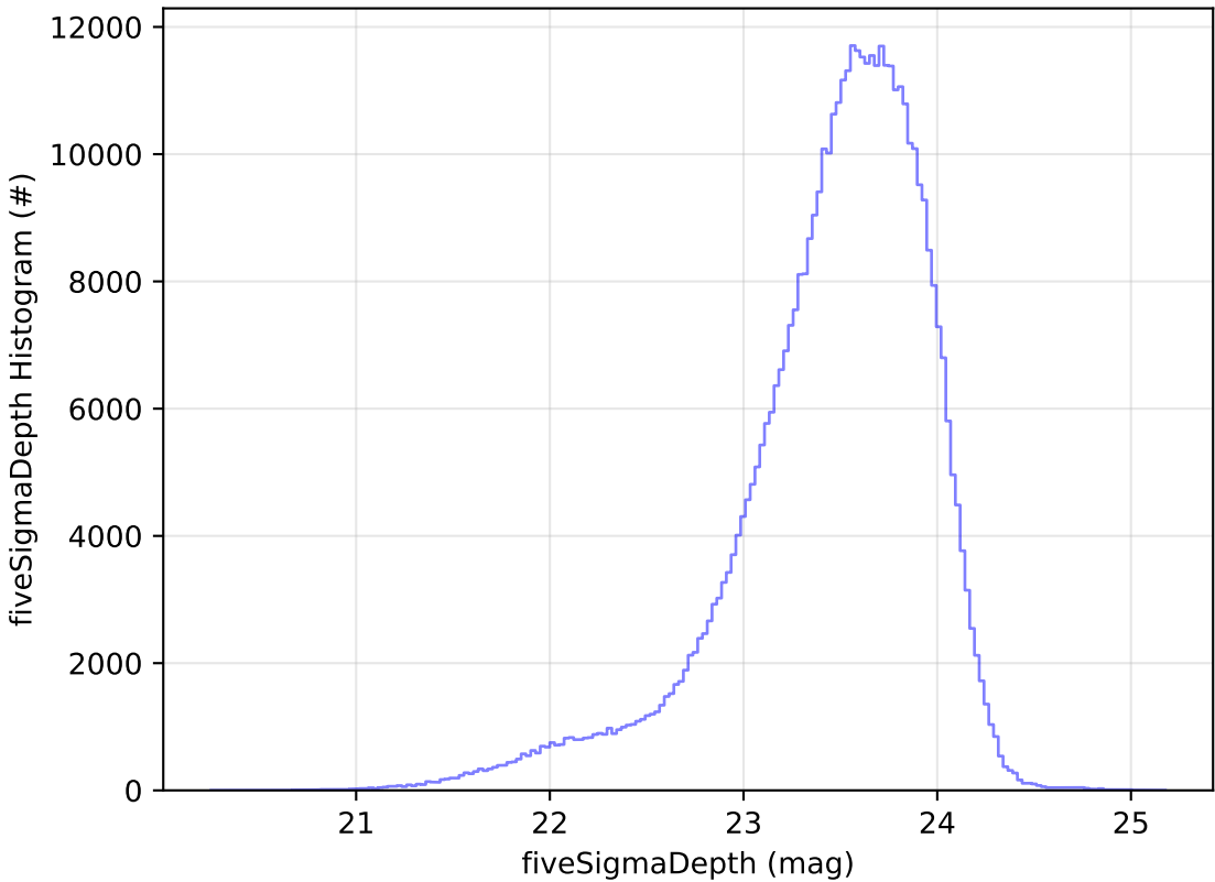
too_combined_s0.5_v3.4_10yrs i: fiveSigmaDepth Histogram
