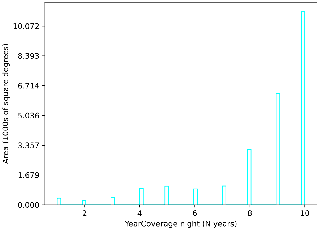
too_combined_s0.5_v3.4_10yrs u band: YearCoverage night
