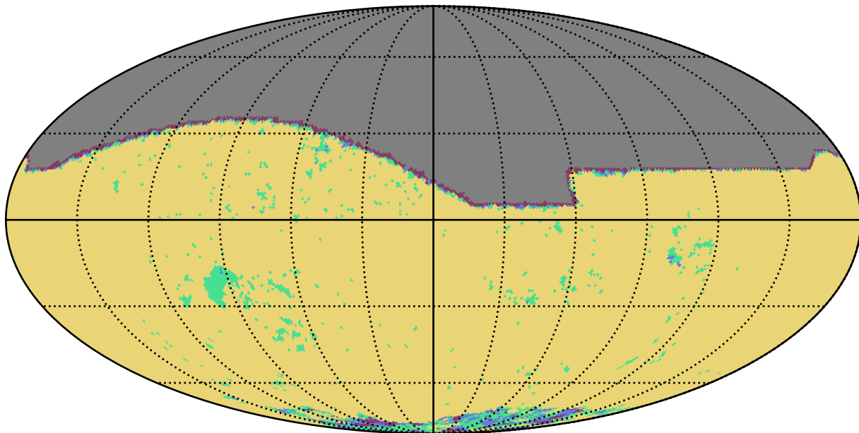
too_combined_s0.5_v3.4_10yrs i band: YearCoverage night
