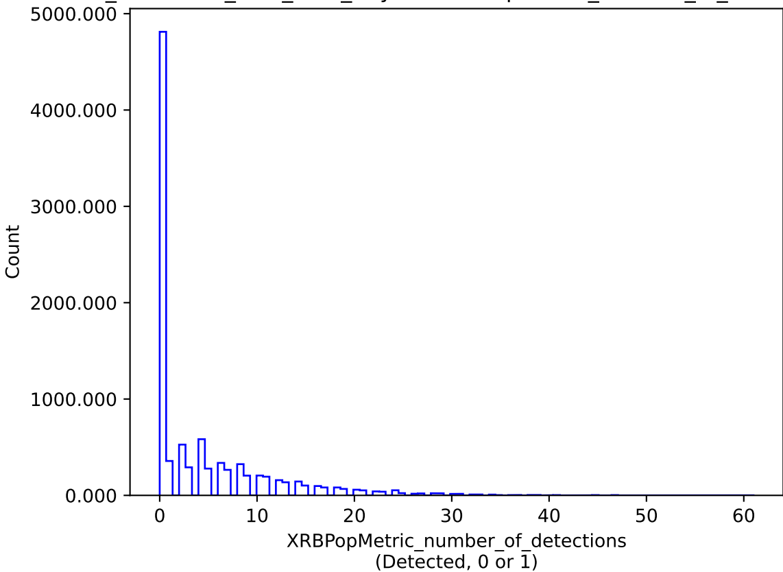
too_combined_s0.5_v3.4_10yrs : XRBPoMetric_number_of_detections
