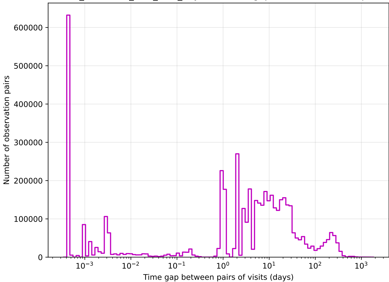
too_combined_s0.5_v3.4_10yrs z band: Tgaps observationStartMJD
