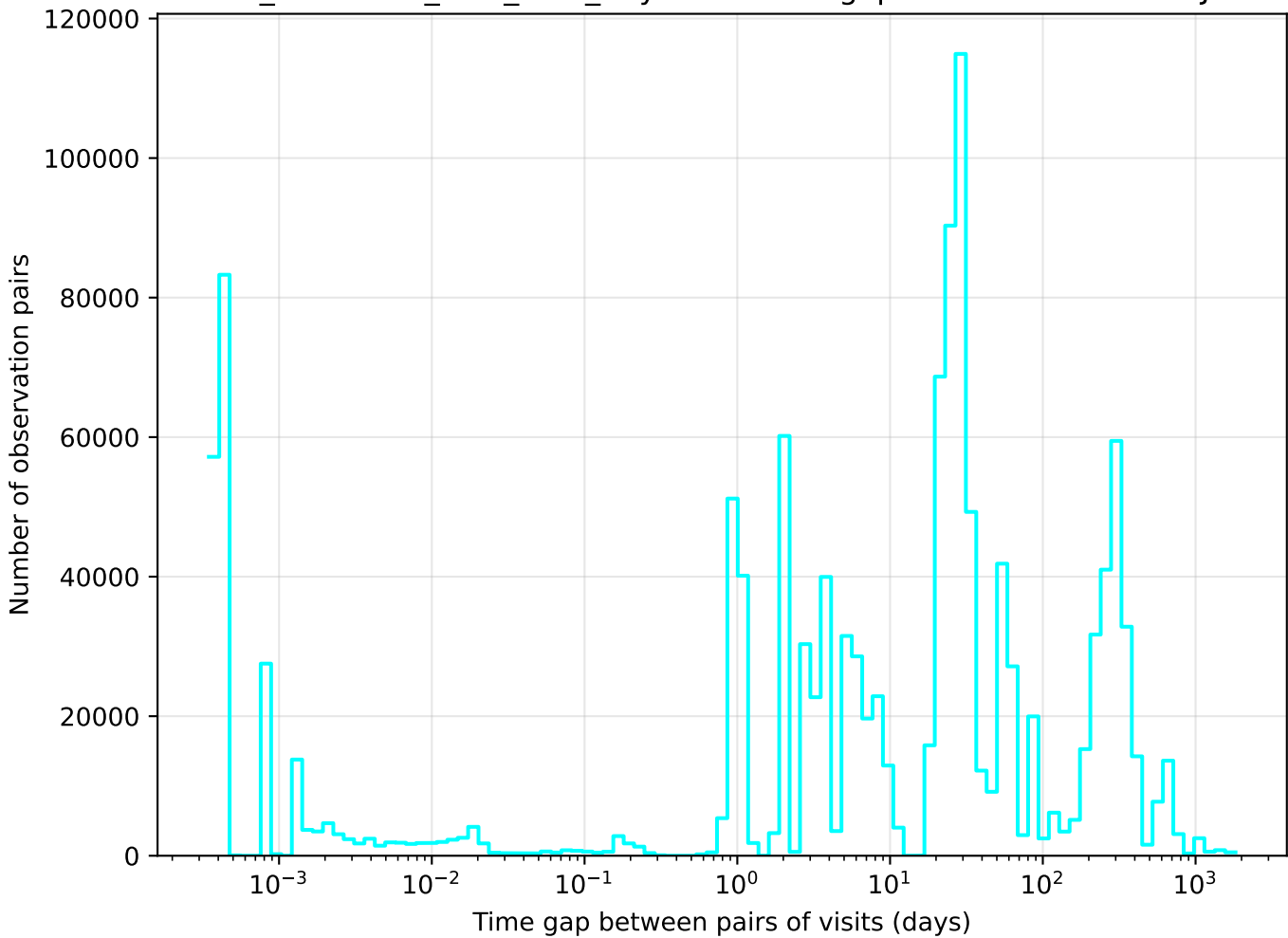
too_combined_s0.5_v3.4_10yrs u band: Tgaps observationStartMJD
