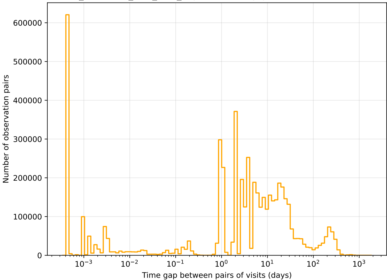
too_combined_s0.5_v3.4_10yrs r band: Tgaps observationStartMJD
