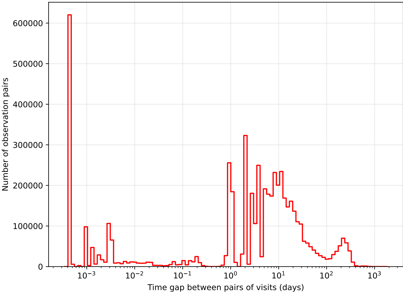
too_combined_s0.5_v3.4_10yrs i band: Tgaps observationStartMJD
