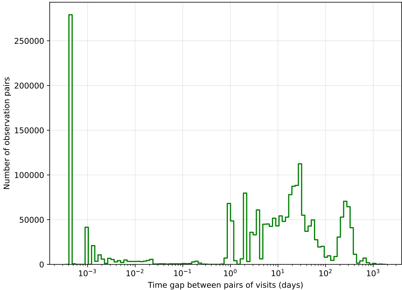
too_combined_s0.5_v3.4_10yrs g band: Tgaps observationStartMJD
