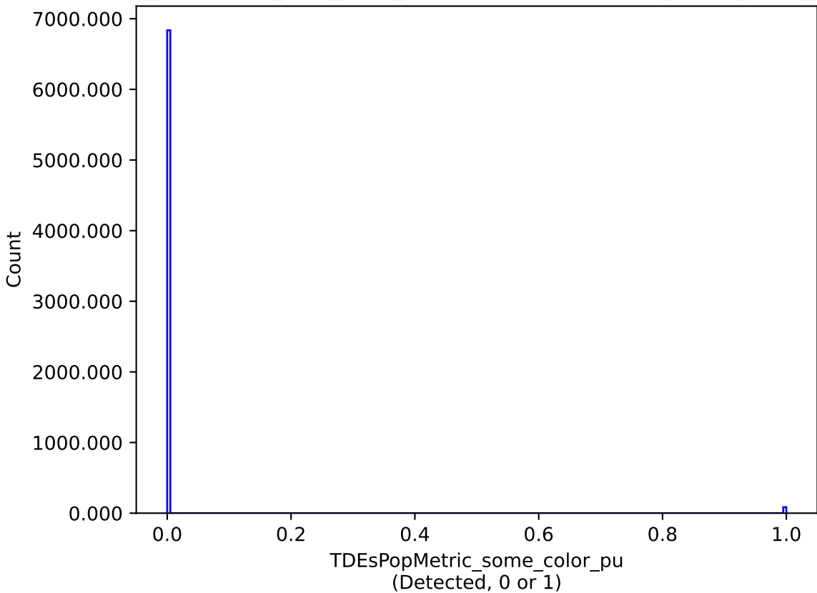
too_combined_s0.5_v3.4_10yrs : TDEsPopMetric_some_color_pu
