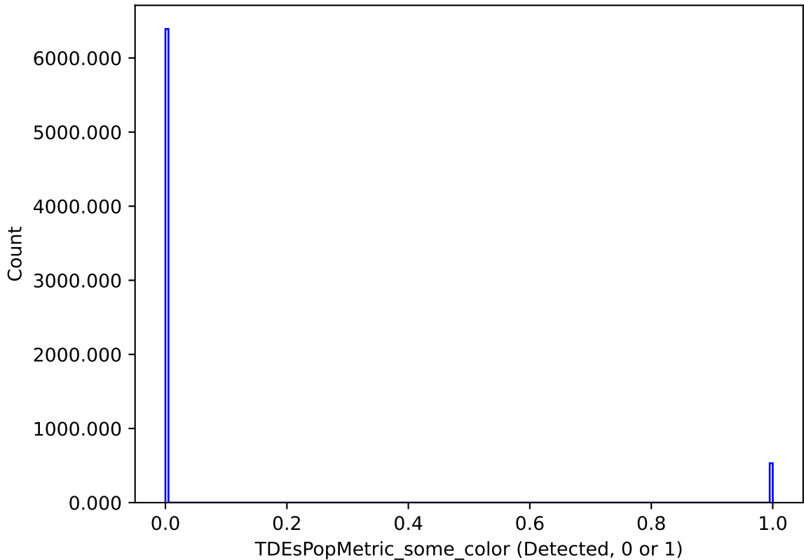
too_combined_s0.5_v3.4_10yrs : TDEsPopMetric_some_color
