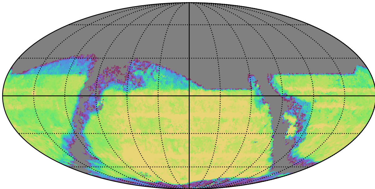
too_combined_s0.5_v3.4_10yrs : TDC_season
