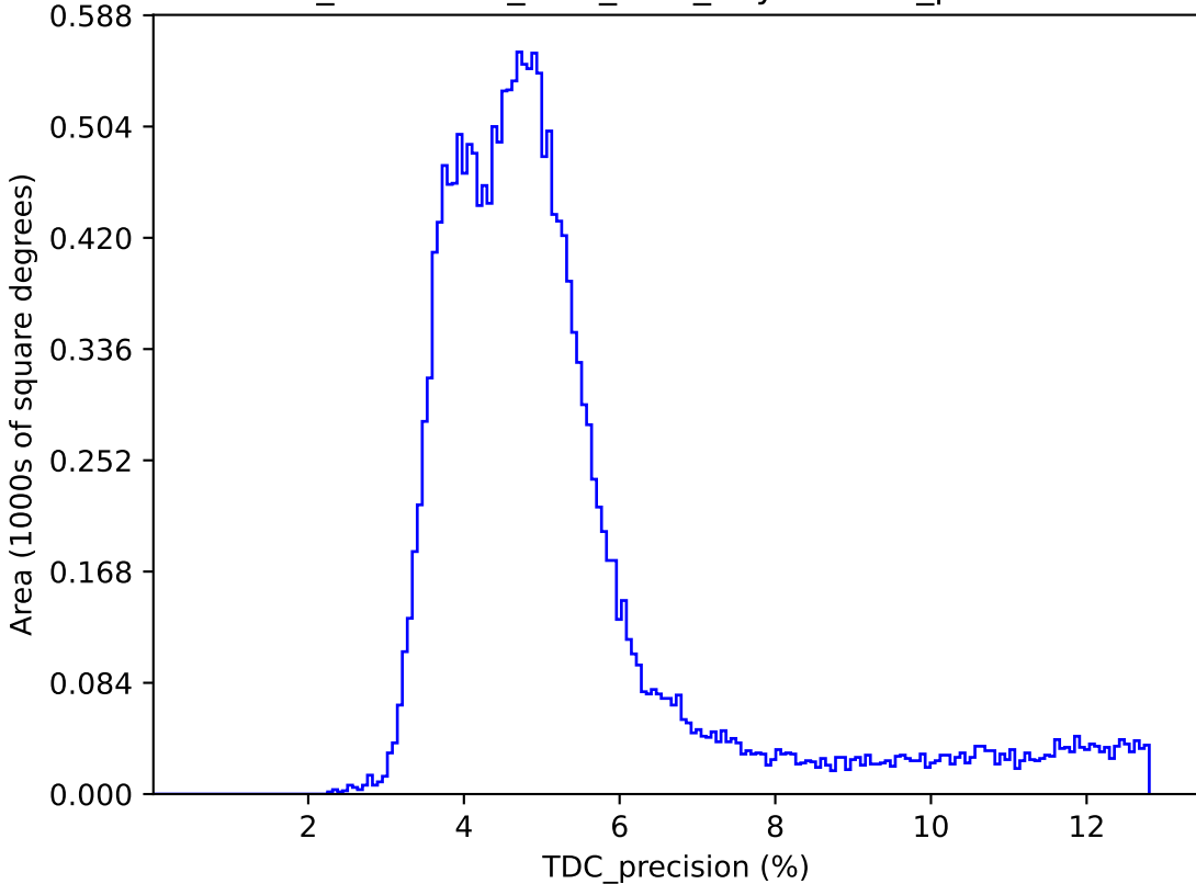
too_combined_s0.5_v3.4_10yrs : TDC_precision
