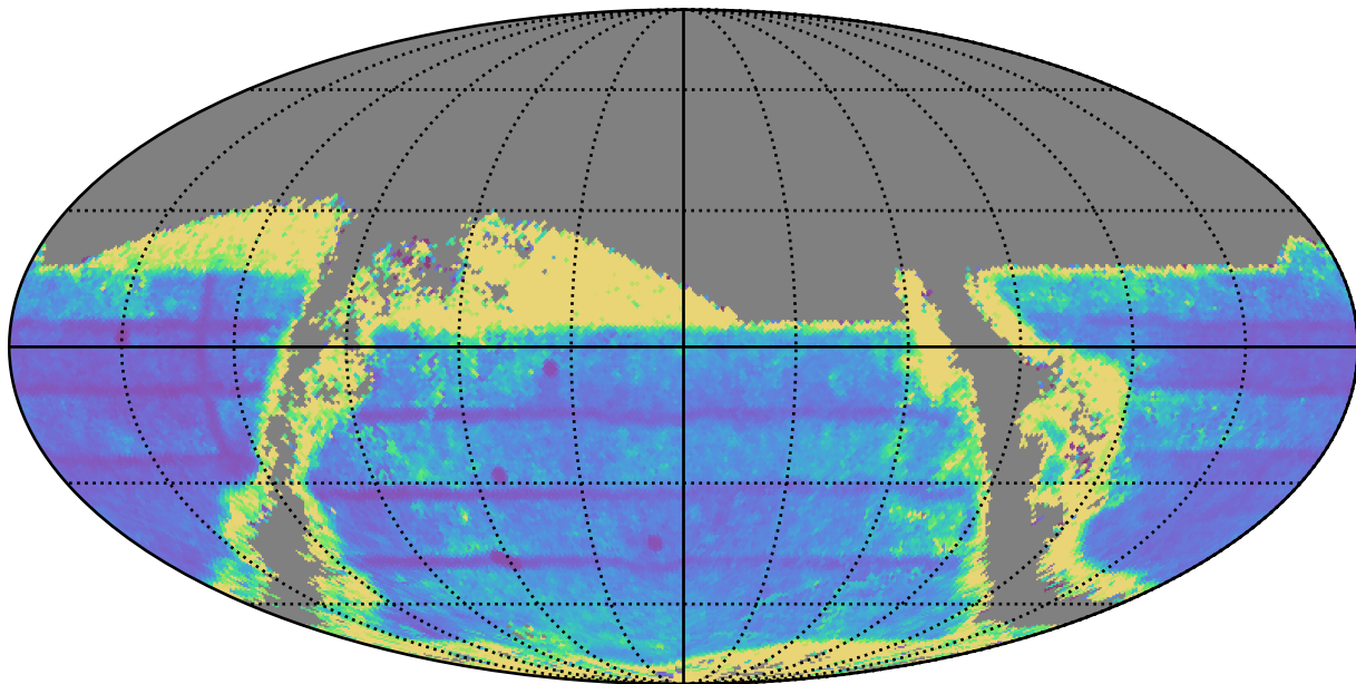
too_combined_s0.5_v3.4_10yrs : TDC_cadence
