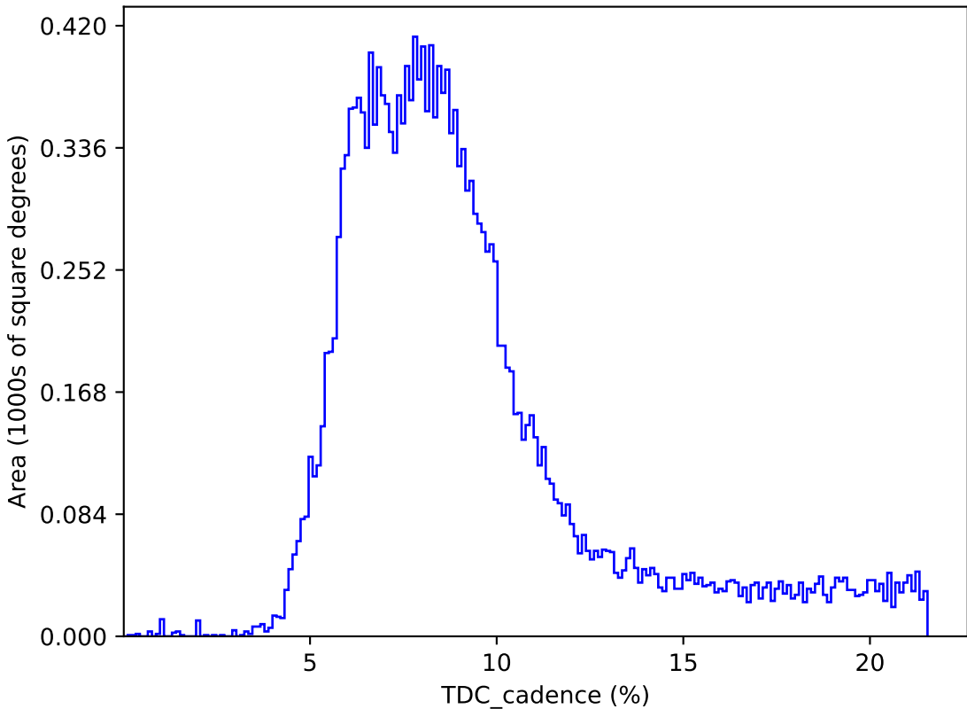
too_combined_s0.5_v3.4_10yrs : TDC_cadence
