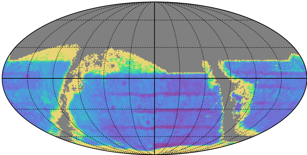
too_combined_s0.5_v3.4_10yrs : TDC_accuracy
