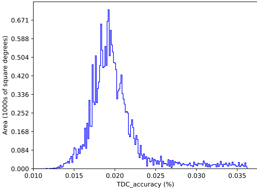
too_combined_s0.5_v3.4_10yrs : TDC_accuracy
