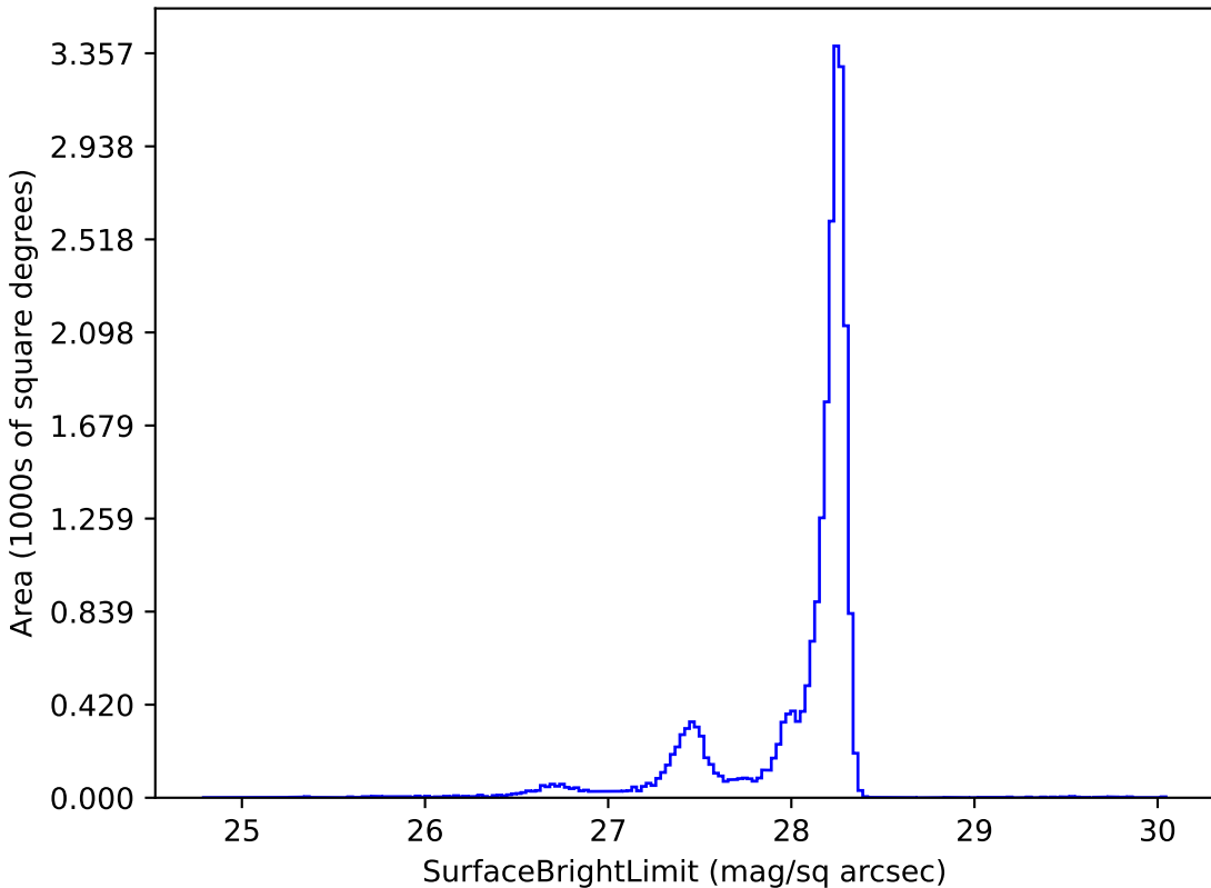
too_combined_s0.5_v3.4_10yrs y: SurfaceBrightLimit
