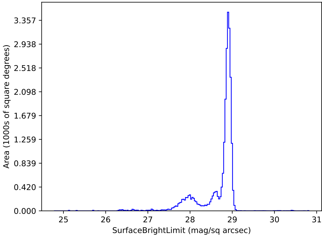
too_combined_s0.5_v3.4_10yrs u: SurfaceBrightLimit
