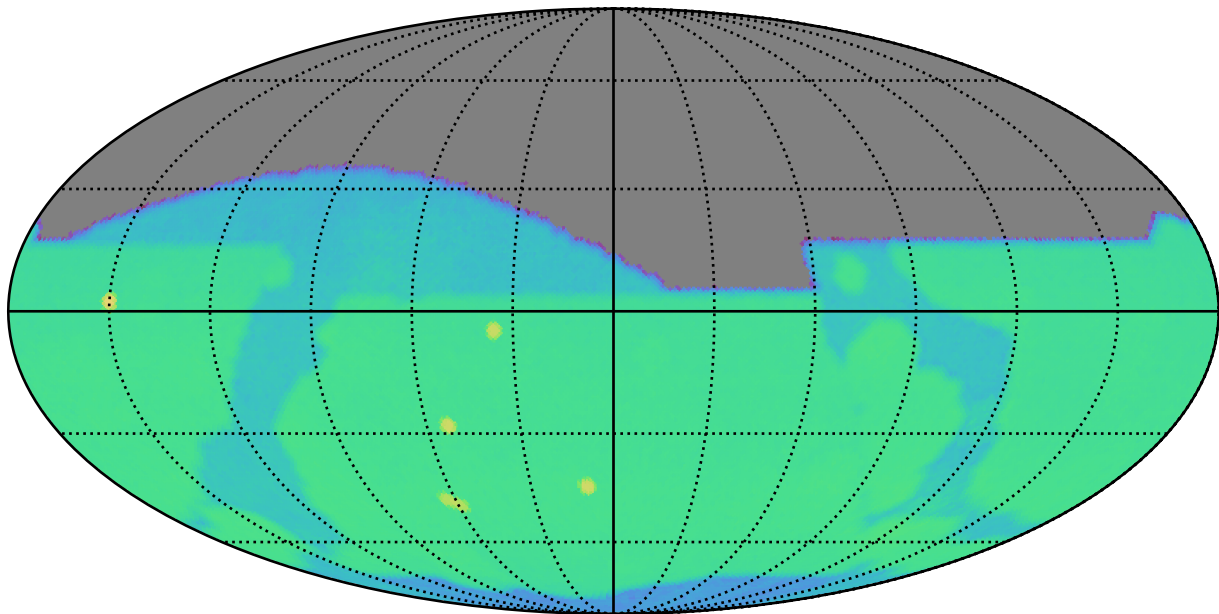
too_combined_s0.5_v3.4_10yrs r: SurfaceBrightLimit
