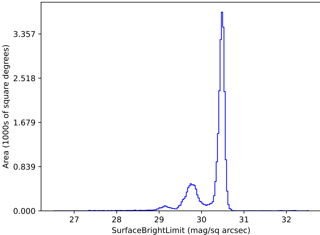
too_combined_s0.5_v3.4_10yrs r: SurfaceBrightLimit
