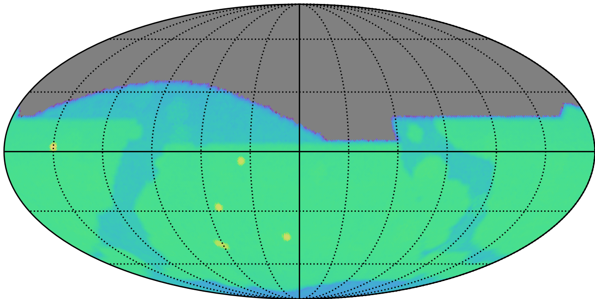
too_combined_s0.5_v3.4_10yrs i: SurfaceBrightLimit
