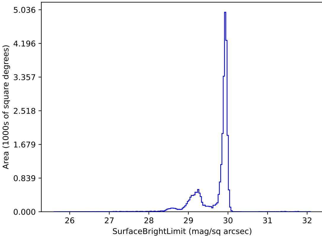
too_combined_s0.5_v3.4_10yrs i: SurfaceBrightLimit
