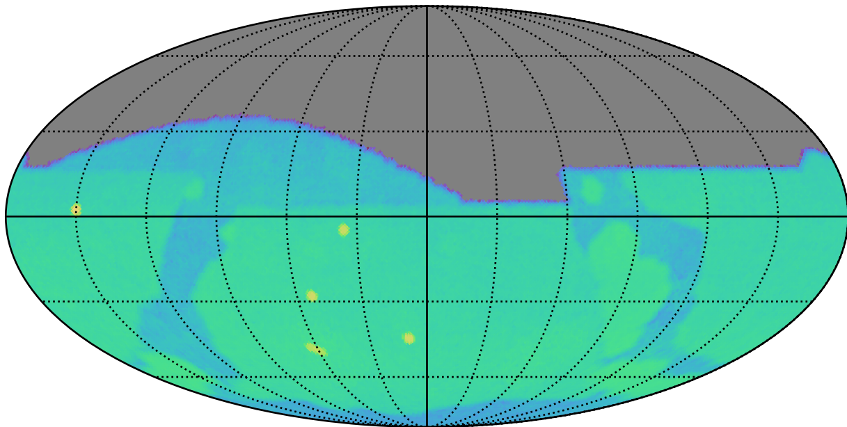
too_combined_s0.5_v3.4_10yrs g: SurfaceBrightLimit
