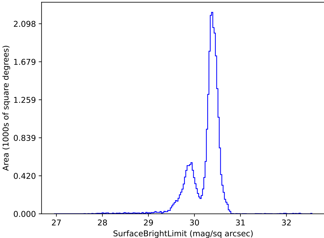
too_combined_s0.5_v3.4_10yrs g: SurfaceBrightLimit
