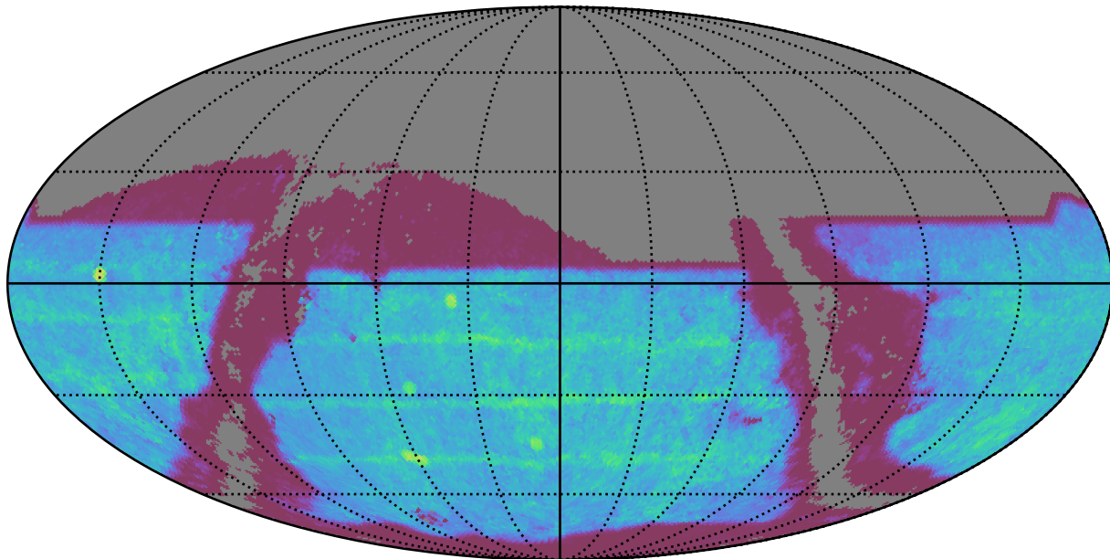
too_combined_s0.5_v3.4_10yrs : SNSLMetric
