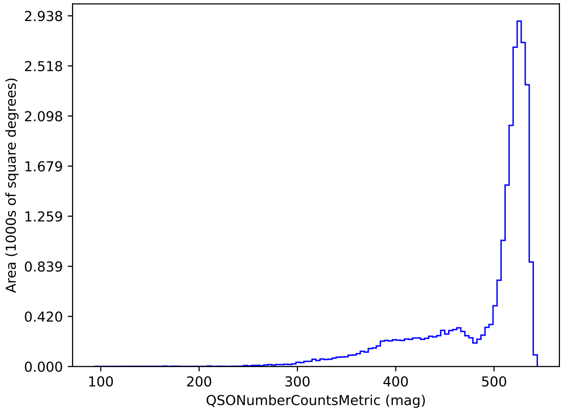
too_combined_s0.5_v3.4_10yrs r band and non-DD: QSONumberCountsMetric
