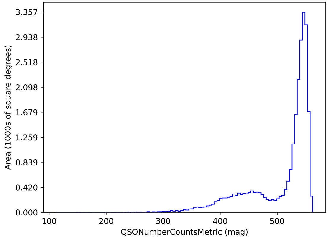
too_combined_s0.5_v3.4_10yrs i band and non-DD: QSONumberCountsMetric
