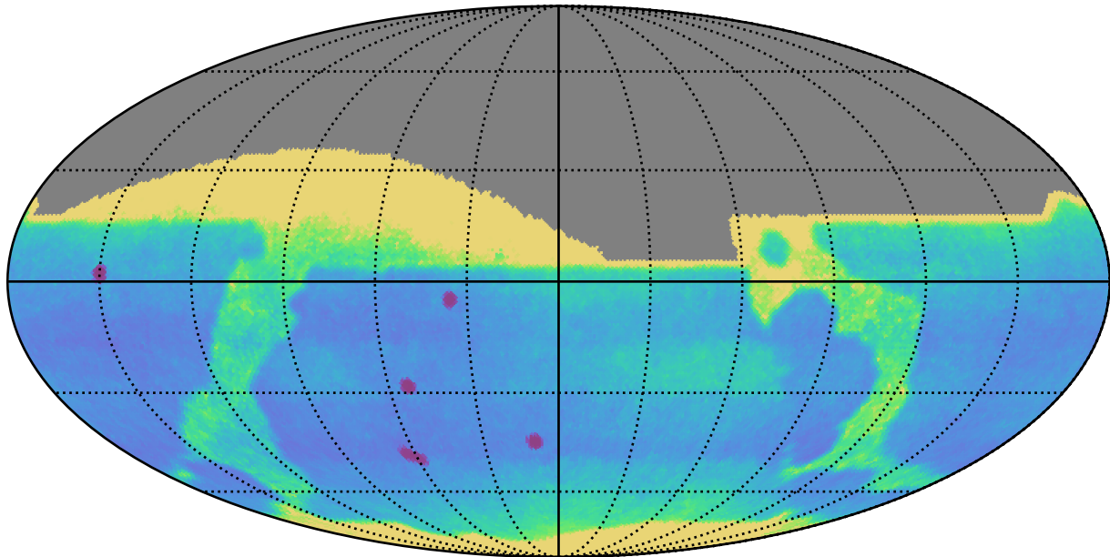
too_combined_s0.5_v3.4_10yrs : Proper Motion Uncert @ 24.0
