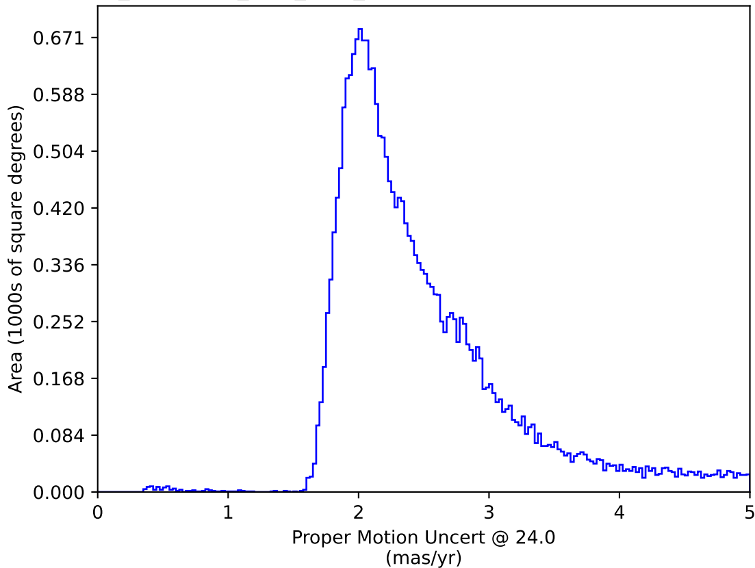
too_combined_s0.5_v3.4_10yrs : Proper Motion Uncert @ 24.0
