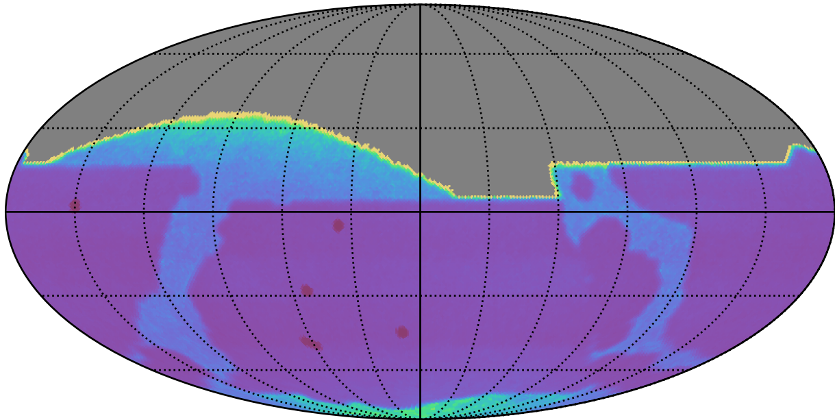
too_combined_s0.5_v3.4_10yrs : Proper Motion Uncert @ 20.5
