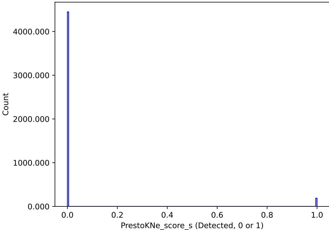
too_combined_s0.5_v3.4_10yrs : PrestoKNe_score_s
