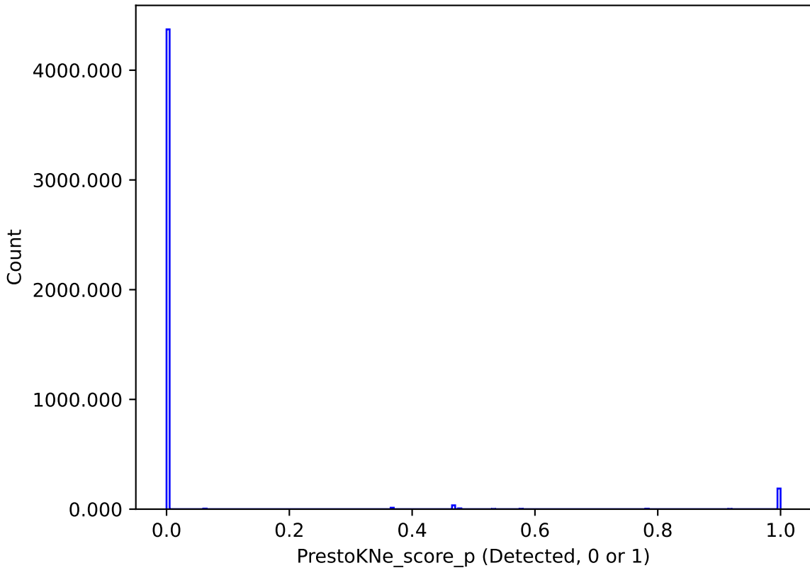
too_combined_s0.5_v3.4_10yrs : PrestoKNe_score_p
