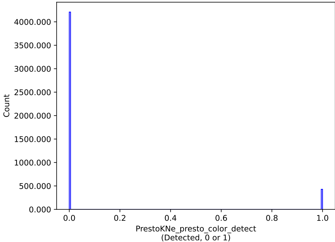
too_combined_s0.5_v3.4_10yrs : PrestoKNe_presto_color_detect
