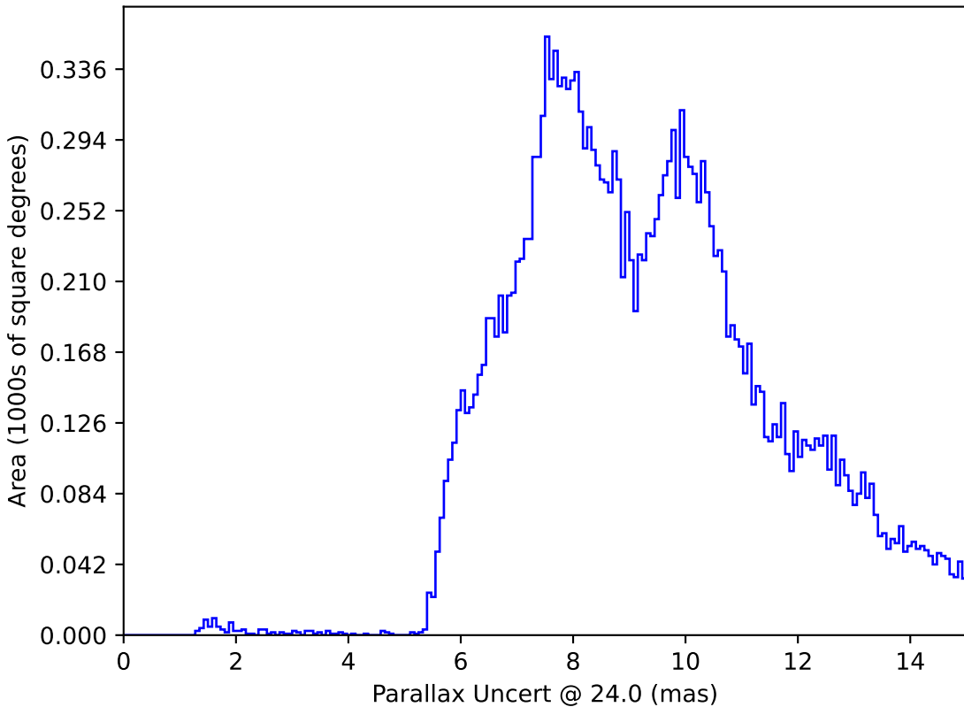
too_combined_s0.5_v3.4_10yrs : Parallax Uncert @ 24.0
