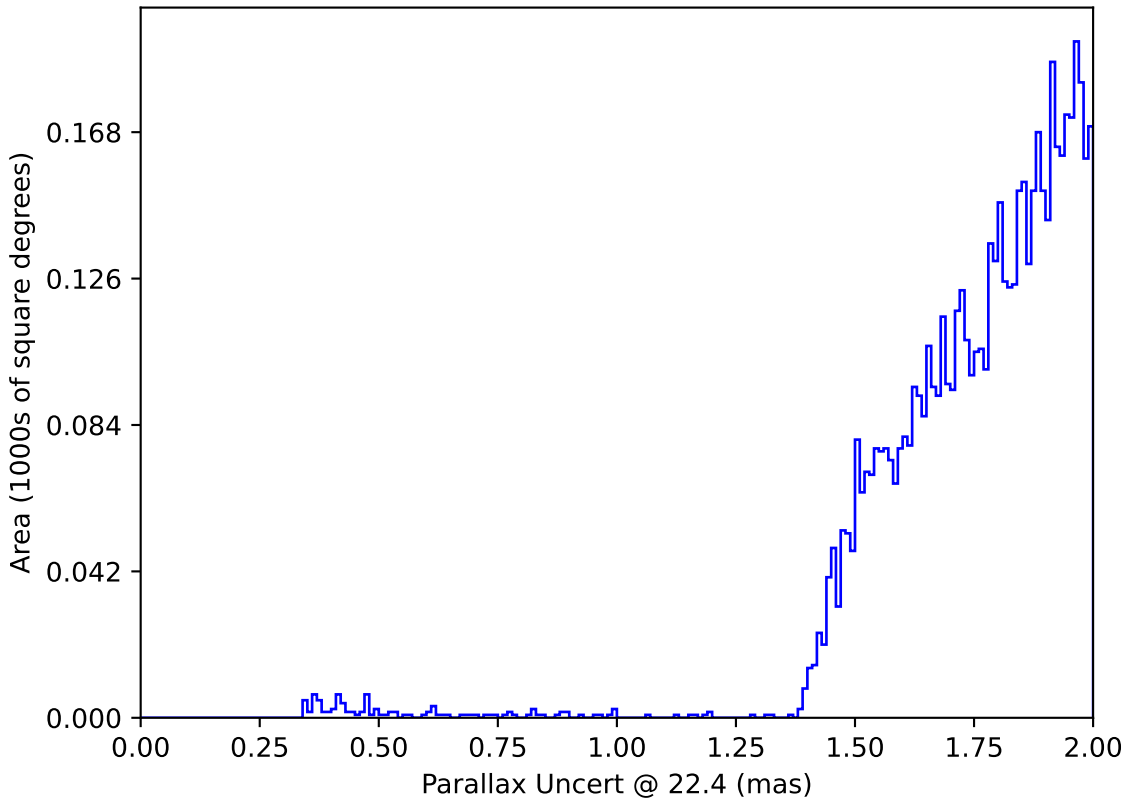
too_combined_s0.5_v3.4_10yrs : Parallax Uncert @ 22.4
