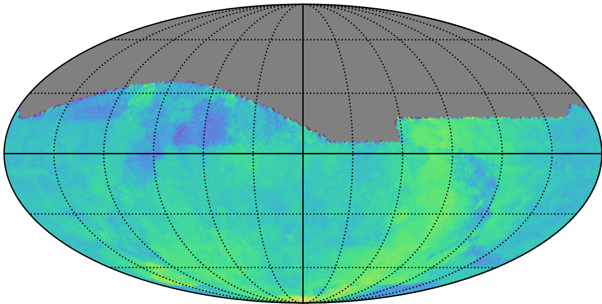
too_combined_s0.5_v3.4_10yrs : Parallax Coverage @ 24.0
