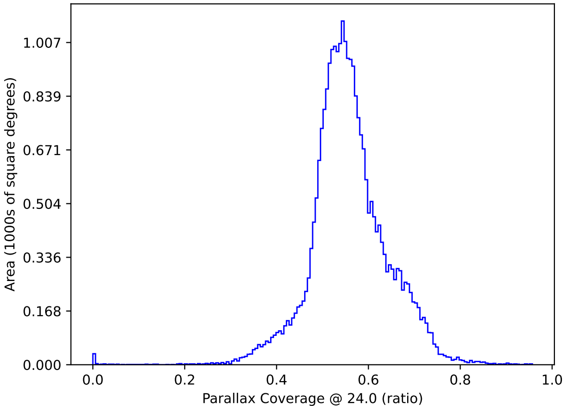
too_combined_s0.5_v3.4_10yrs : Parallax Coverage @ 24.0
