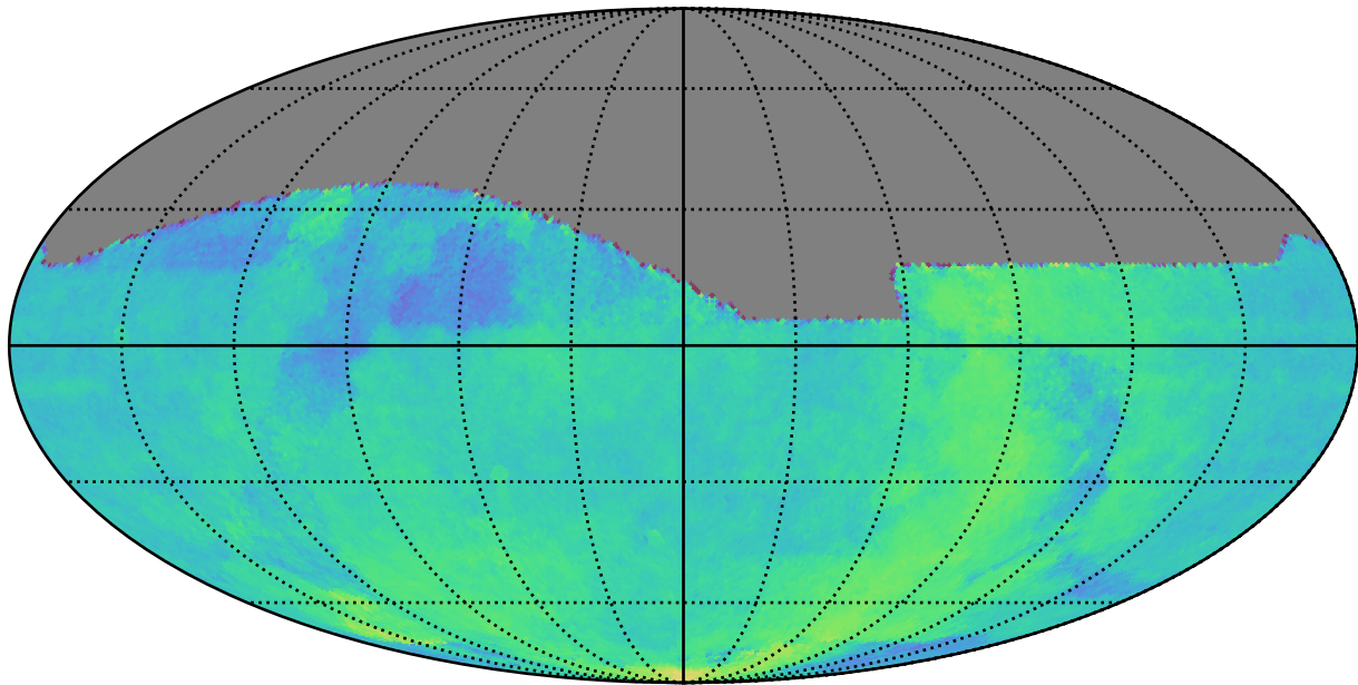
too_combined_s0.5_v3.4_10yrs : Parallax Coverage @ 22.4
